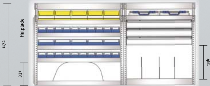
EL-5525 2250 x 992 x 330/430
