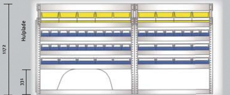
EL-5527 2250 x 992 x 330/430
