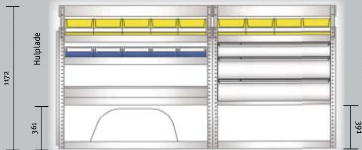
EL-5528 2250 x 992 x 330/430
